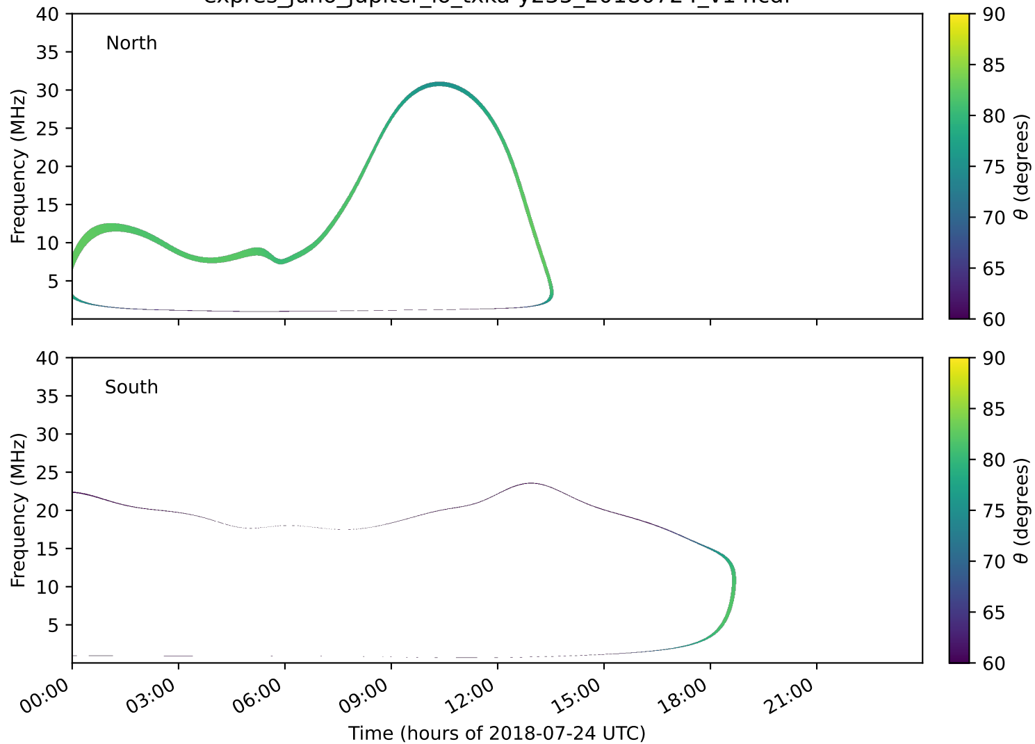
expres_juno_jupiter_io_txka-y235_20180724_v14.cdf
