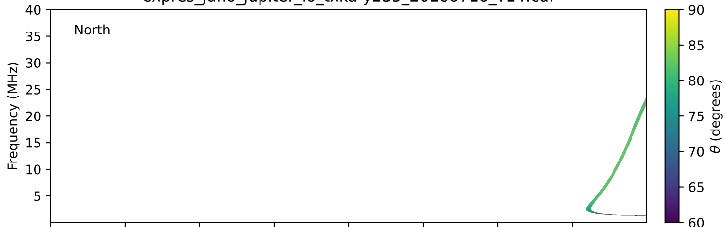
expres_juno_jupiter_io_txka-y235_20180718_v14.cdf
