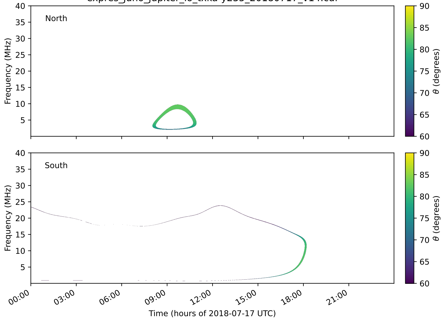
expres_juno_jupiter_io_txka-y235_20180717_v14.cdf
