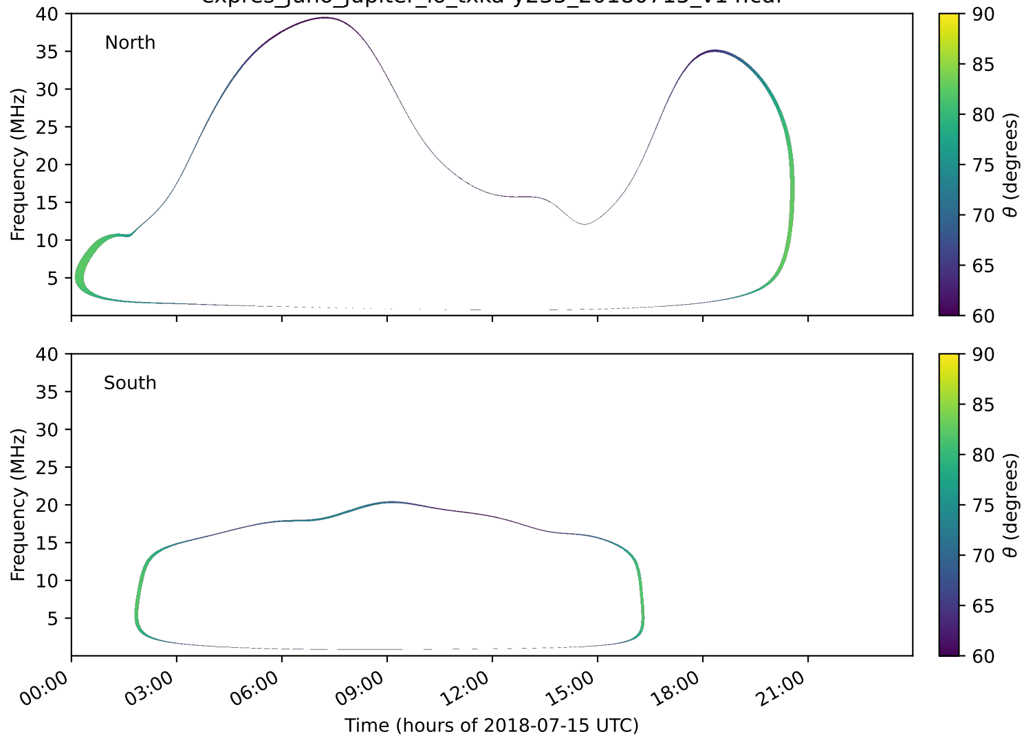
expres_juno_jupiter_io_txka-y235_20180715_v14.cdf
