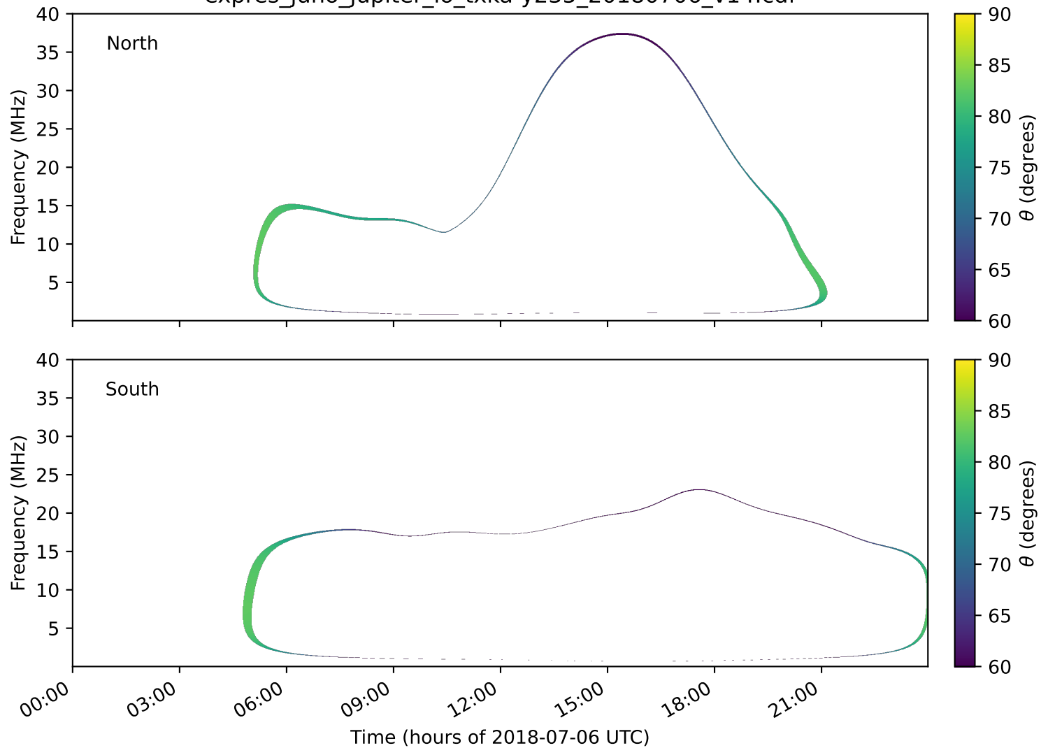
expres_juno_jupiter_io_txka-y235_20180706_v14.cdf
