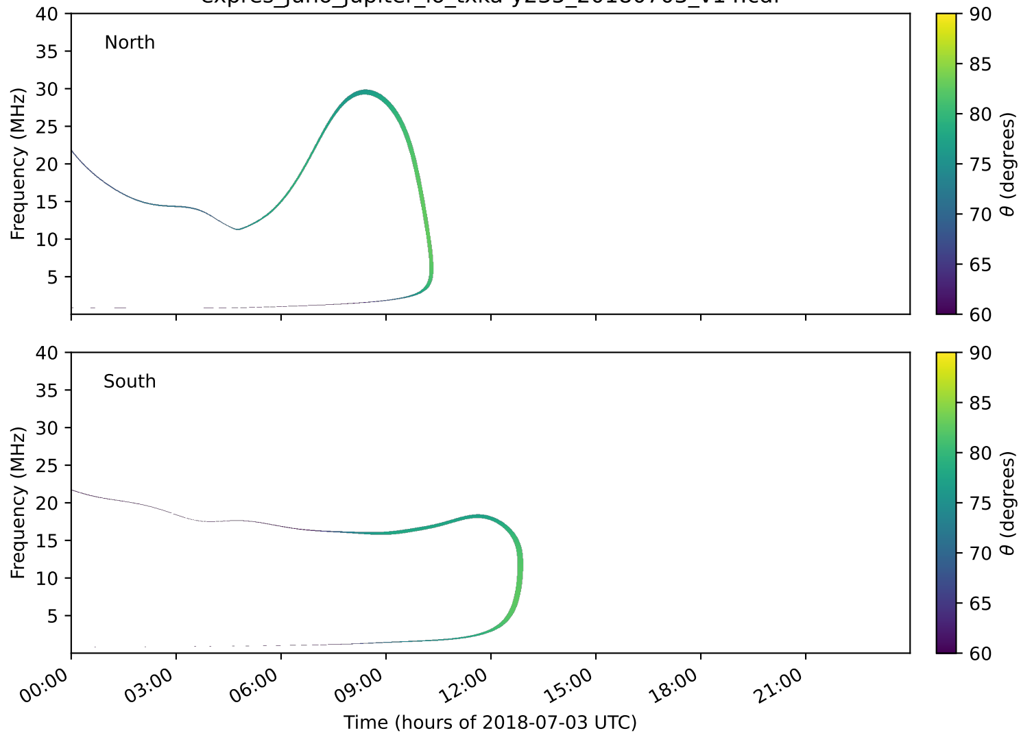
expres_juno_jupiter_io_txka-y235_20180703_v14.cdf
