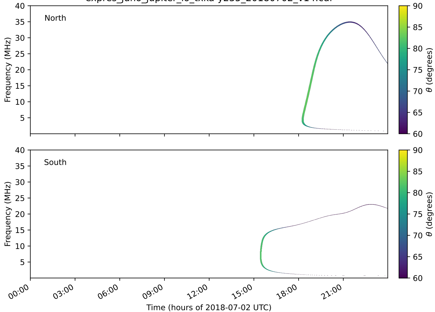
expres_juno_jupiter_io_txka-y235_20180702_v14.cdf
