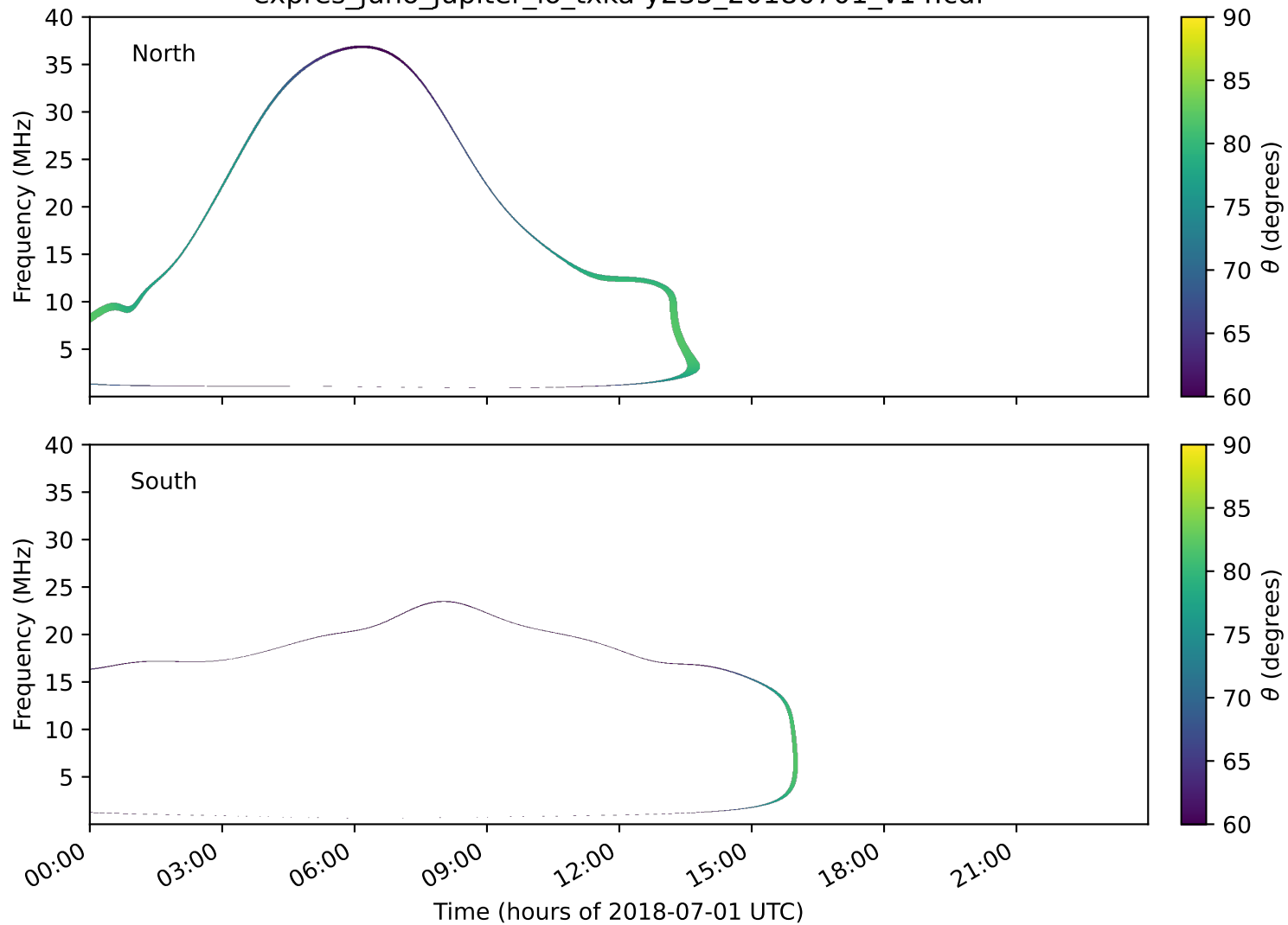
expres_juno_jupiter_io_txka-y235_20180701_v14.cdf
