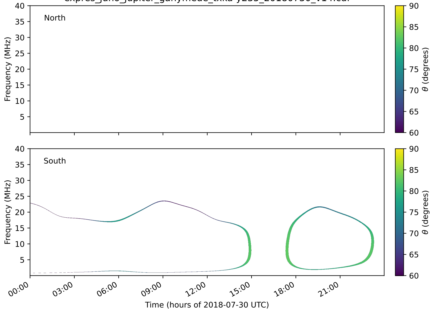
expres_juno_jupiter_ganymede_txka-y235_20180730_v14.cdf
