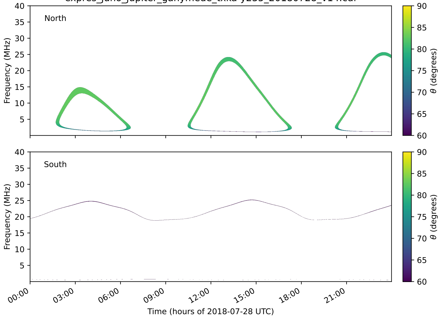
expres_juno_jupiter_ganymede_txka-y235_20180728_v14.cdf
