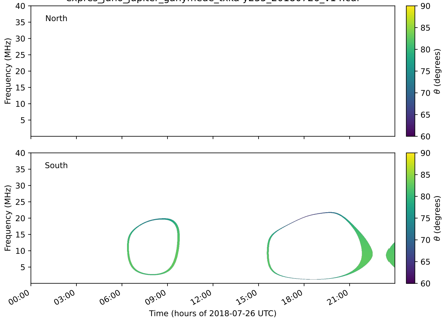
expres_juno_jupiter_ganymede_txka-y235_20180726_v14.cdf
