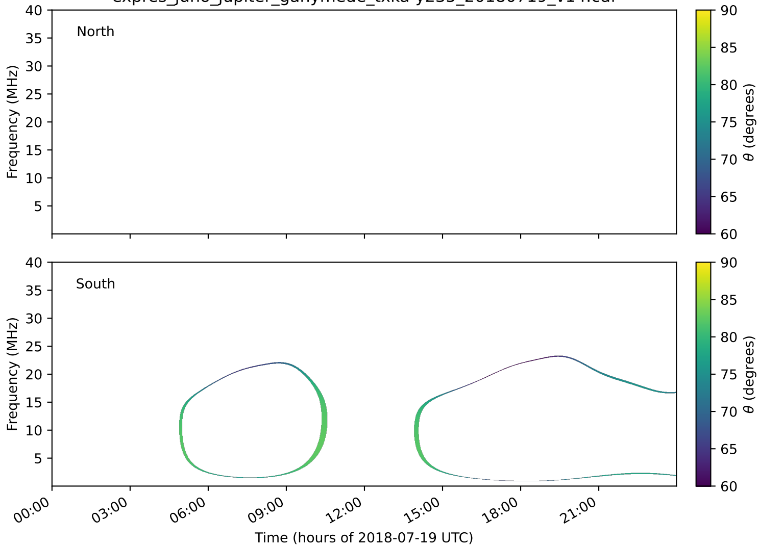
expres_juno_jupiter_ganymede_txka-y235_20180719_v14.cdf
