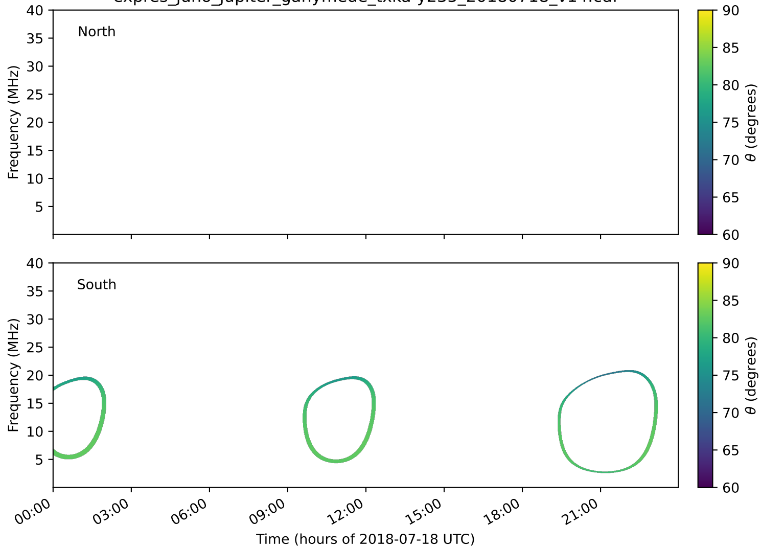
expres_juno_jupiter_ganymede_txka-y235_20180718_v14.cdf
