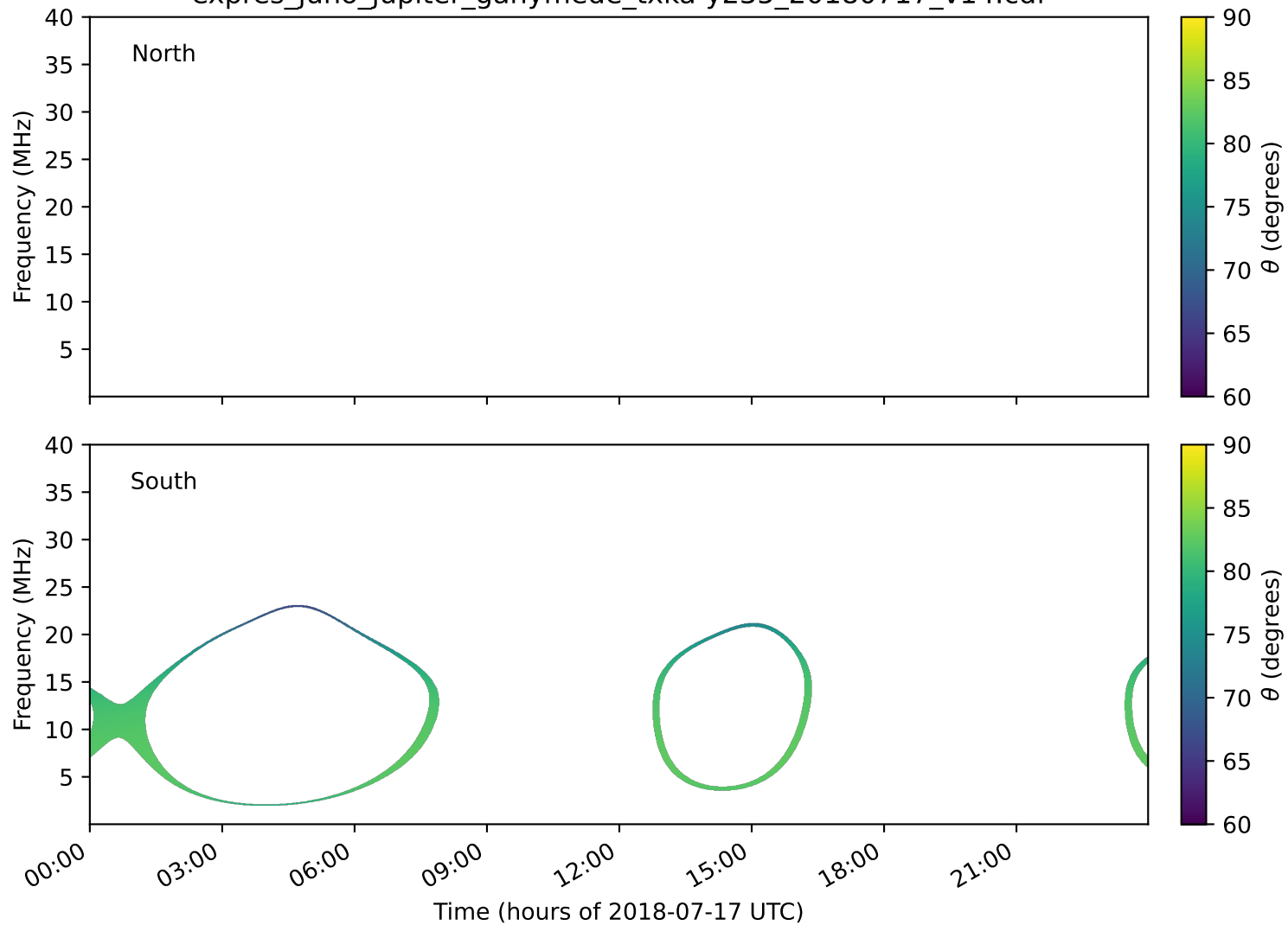
expres_juno_jupiter_ganymede_txka-y235_20180717_v14.cdf
