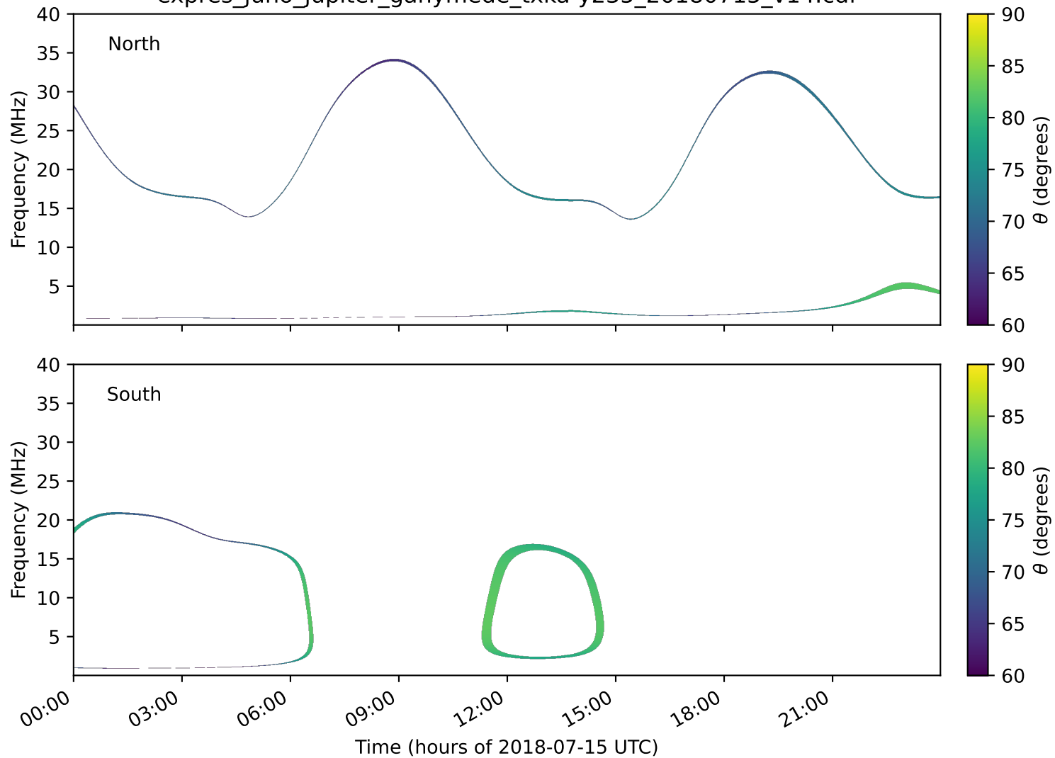
expres_juno_jupiter_ganymede_txka-y235_20180715_v14.cdf
