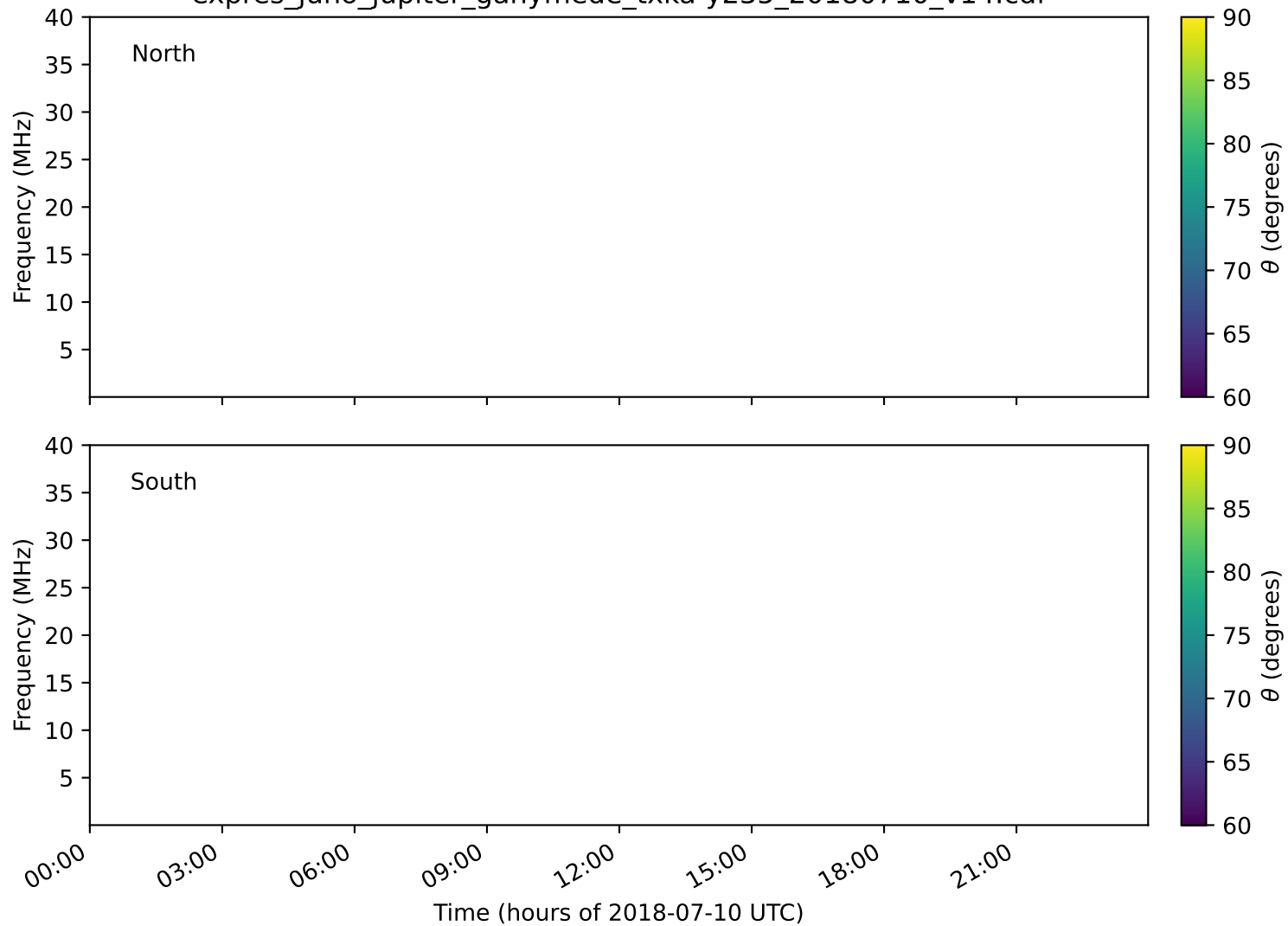
expres_juno_jupiter_ganymede_txka-y235_20180710_v14.cdf
