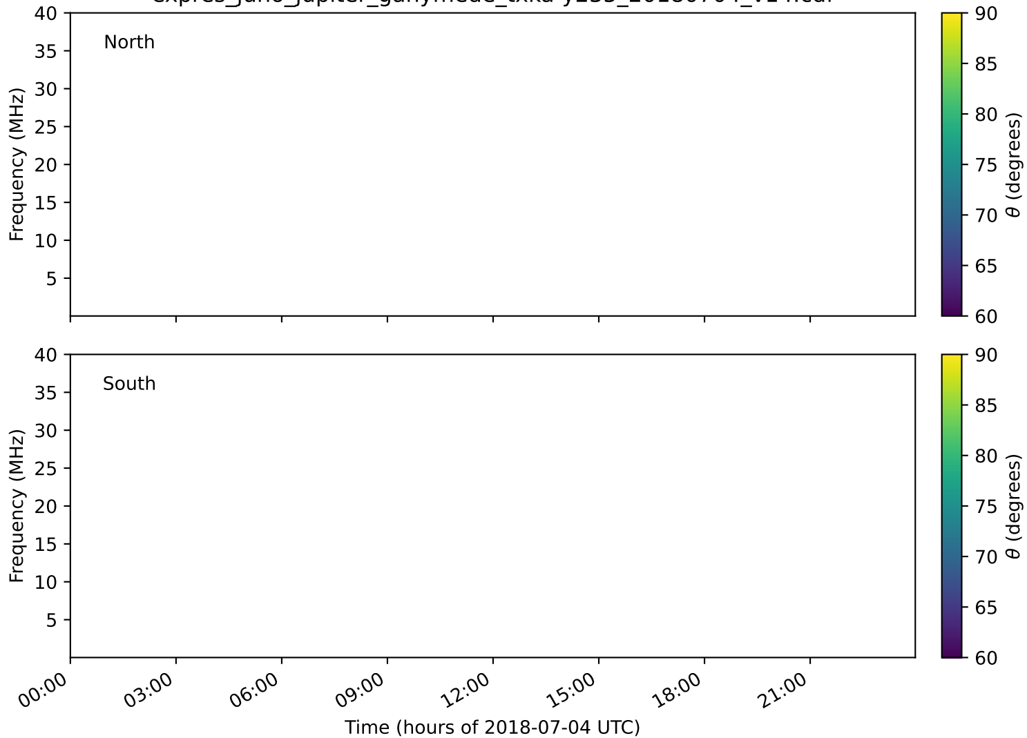
expres_juno_jupiter_ganymede_txka-y235_20180704_v14.cdf
