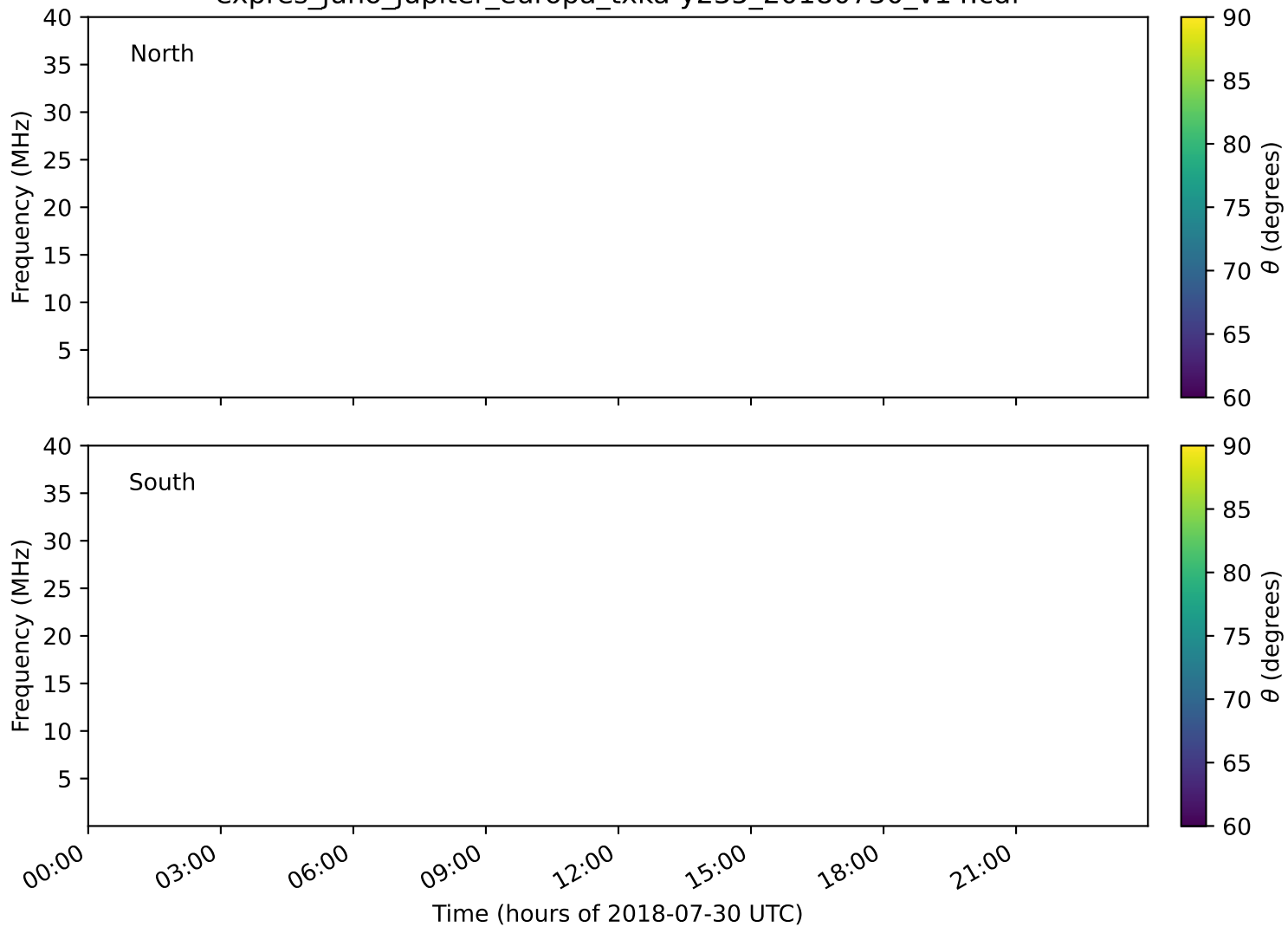
expres_juno_jupiter_europa_txka-y235_20180730_v14.cdf
