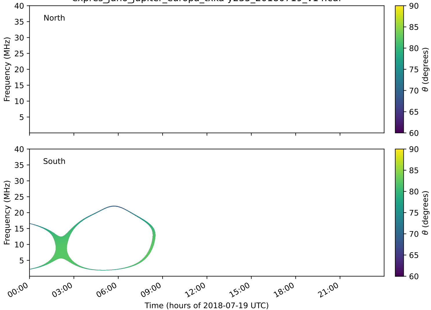
expres_juno_jupiter_europa_txka-y235_20180719_v14.cdf
