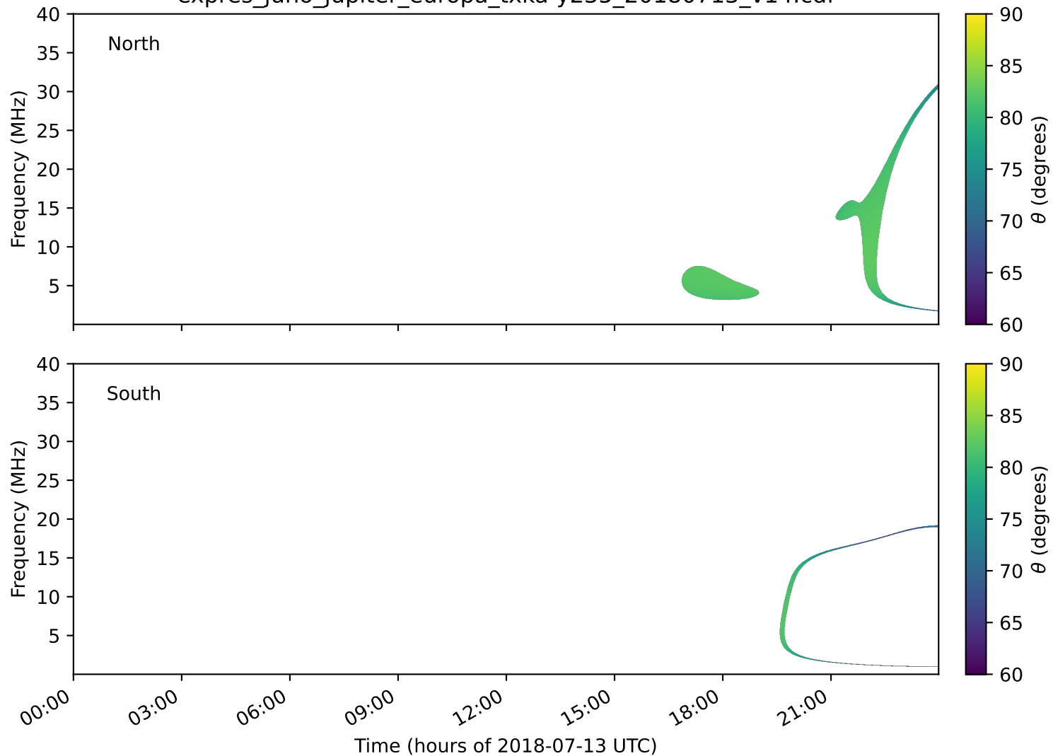
expres_juno_jupiter_europa_txka-y235_20180713_v14.cdf
