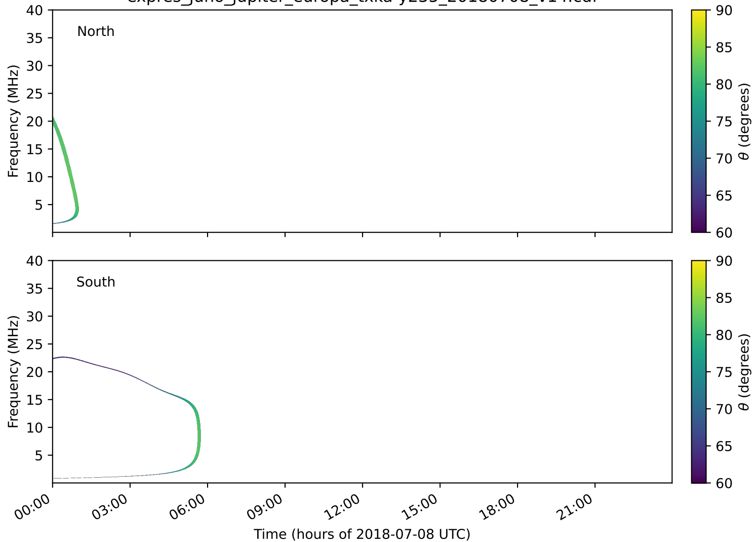
expres_juno_jupiter_europa_txka-y235_20180708_v14.cdf
