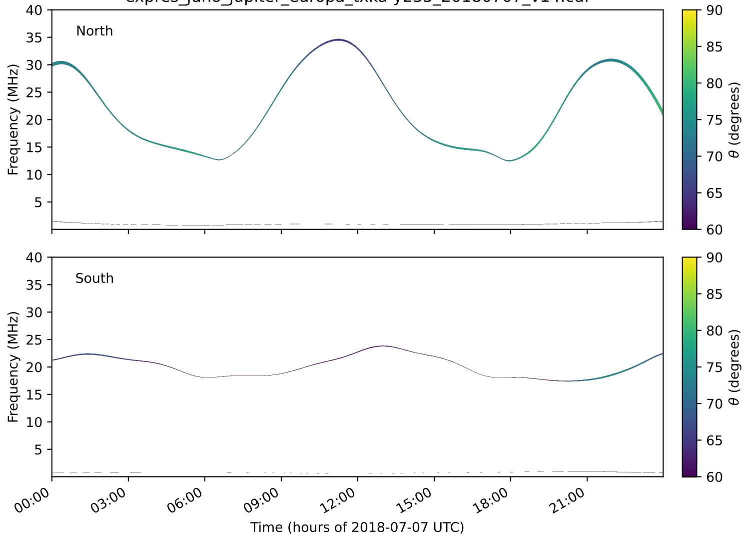
expres_juno_jupiter_europa_txka-y235_20180707_v14.cdf
