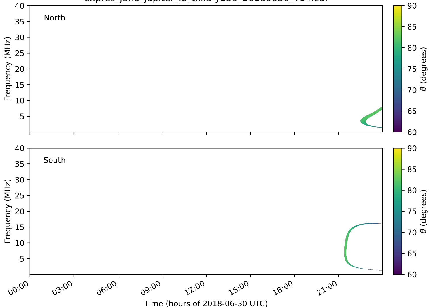
expres_juno_jupiter_io_txka-y235_20180630_v14.cdf
