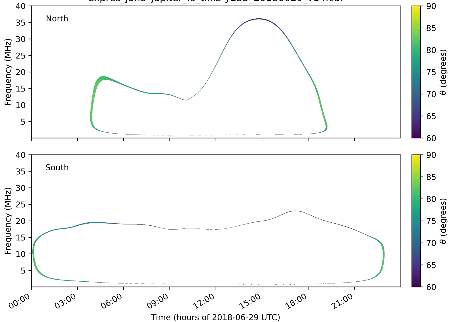
expres_juno_jupiter_io_txka-y235_20180629_v14.cdf
