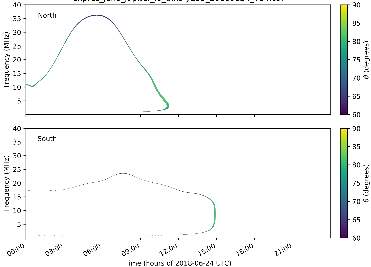
expres_juno_jupiter_io_txka-y235_20180624_v14.cdf
