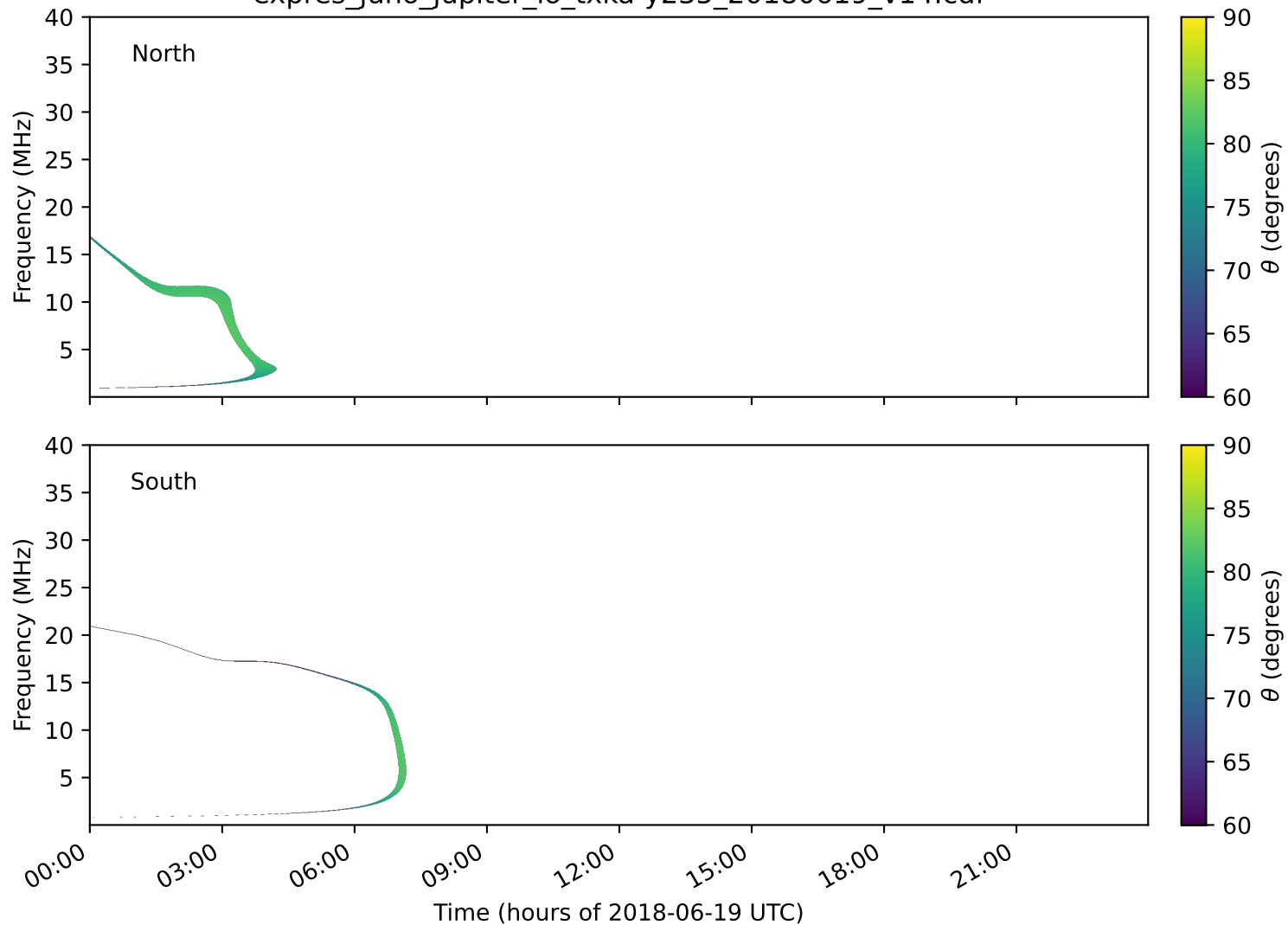
expres_juno_jupiter_io_txka-y235_20180619_v14.cdf
