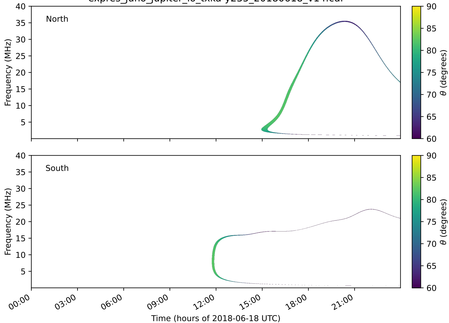
expres_juno_jupiter_io_txka-y235_20180618_v14.cdf
