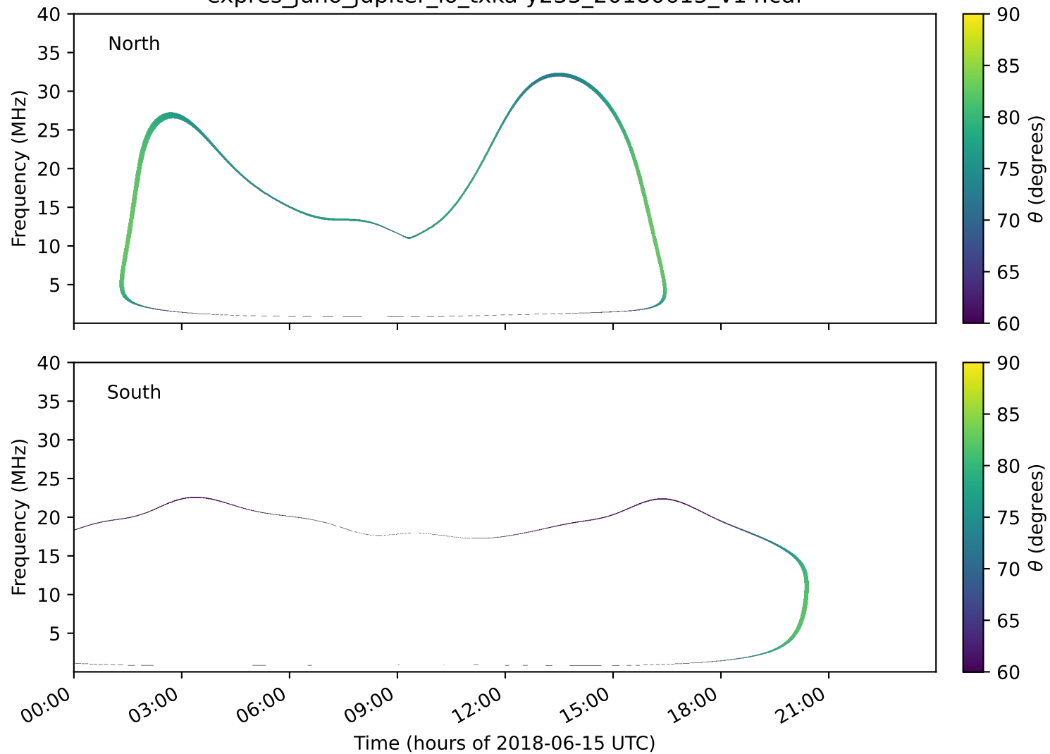
expres_juno_jupiter_io_txka-y235_20180615_v14.cdf
