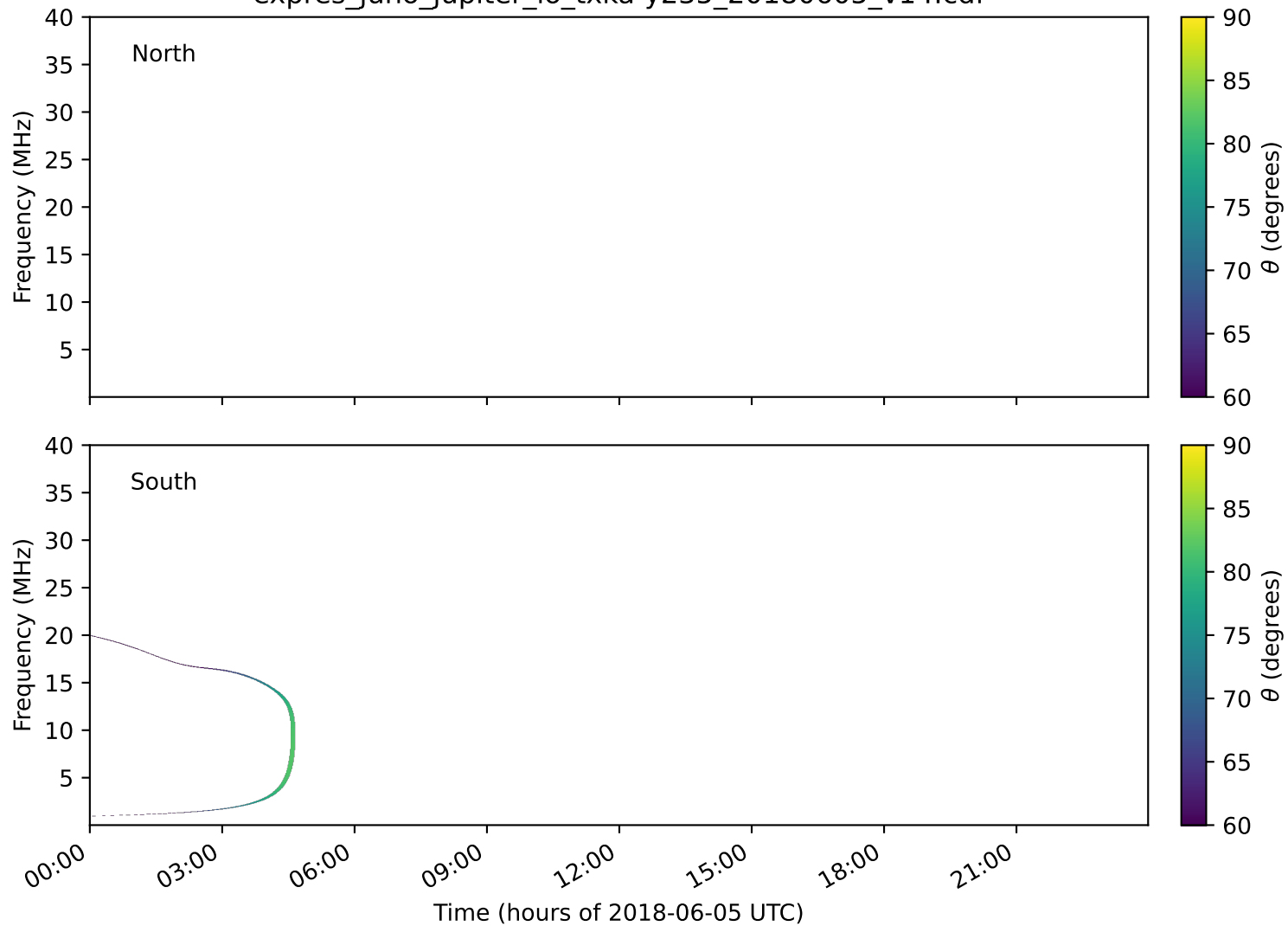
expres_juno_jupiter_io_txka-y235_20180605_v14.cdf
