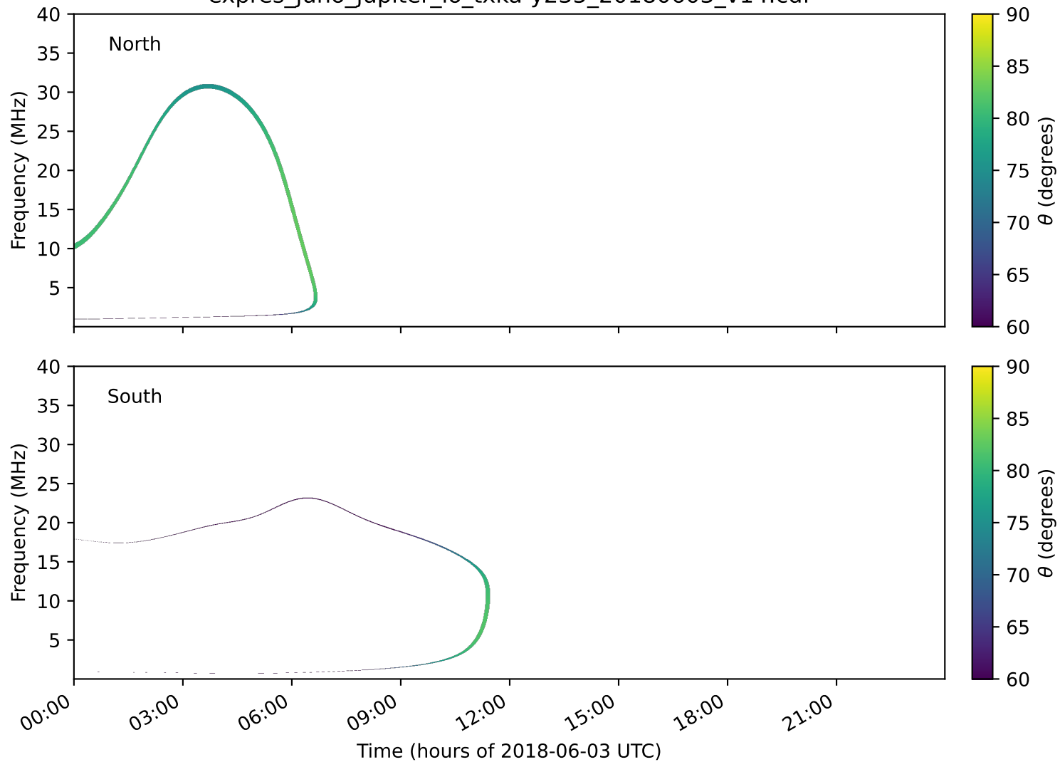
expres_juno_jupiter_io_txka-y235_20180603_v14.cdf
