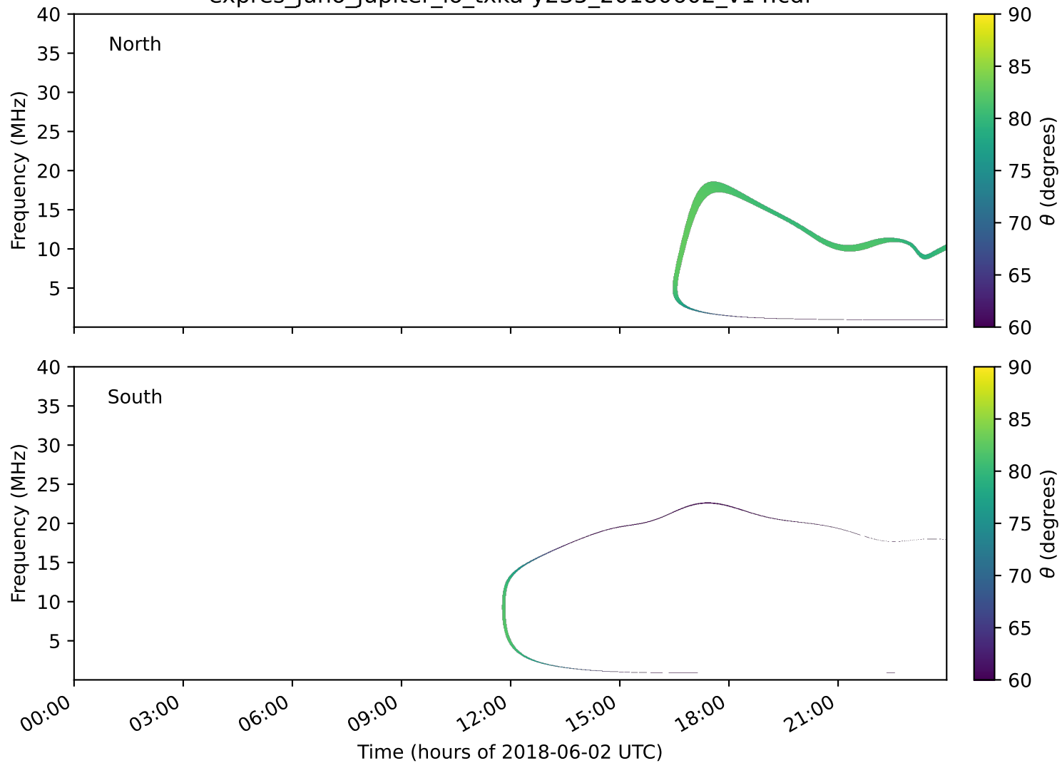
expres_juno_jupiter_io_txka-y235_20180602_v14.cdf
