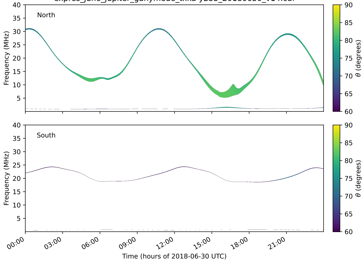
expres_juno_jupiter_ganymede_txka-y235_20180630_v14.cdf
