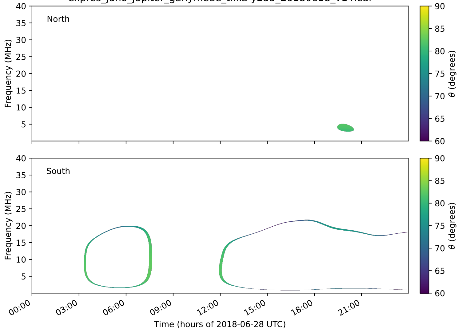
expres_juno_jupiter_ganymede_txka-y235_20180628_v14.cdf
