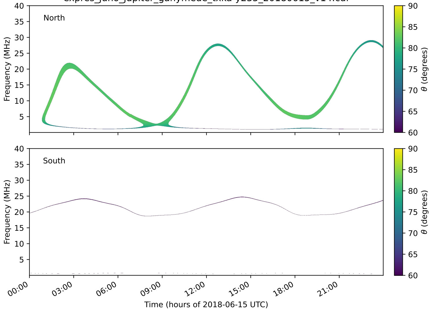
expres_juno_jupiter_ganymede_txka-y235_20180615_v14.cdf
