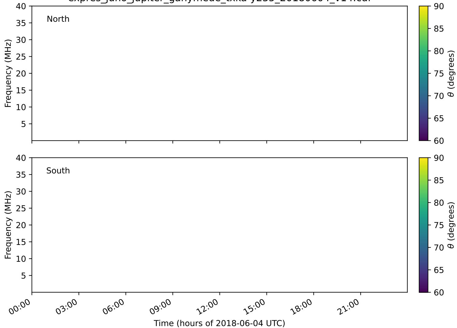
expres_juno_jupiter_ganymede_txka-y235_20180604_v14.cdf
