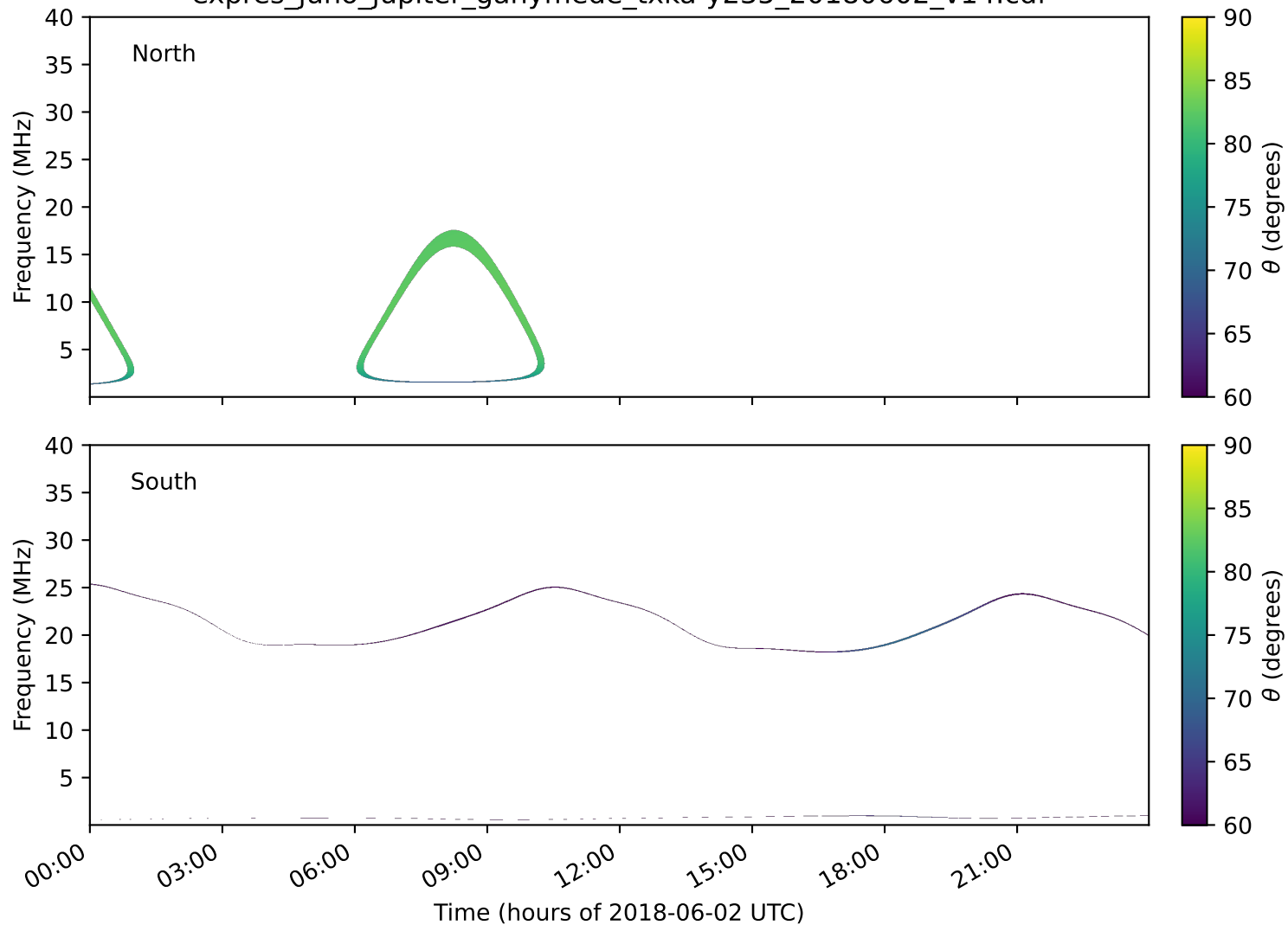
expres_juno_jupiter_ganymede_txka-y235_20180602_v14.cdf
