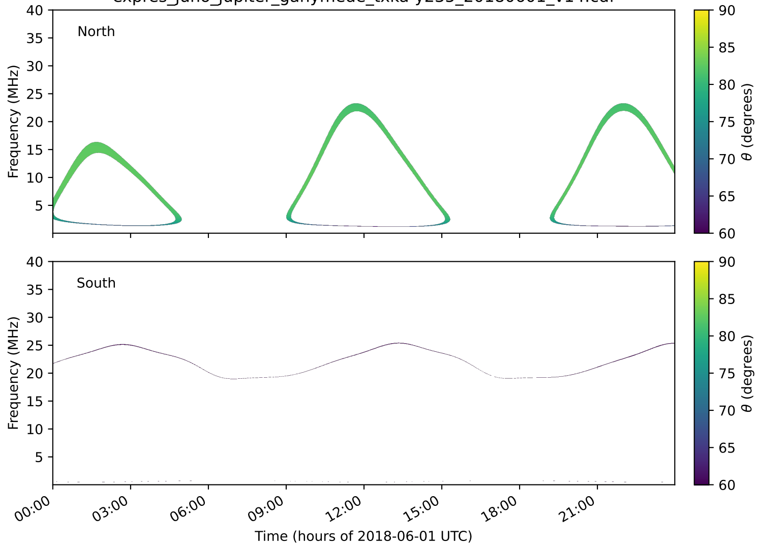
expres_juno_jupiter_ganymede_txka-y235_20180601_v14.cdf
