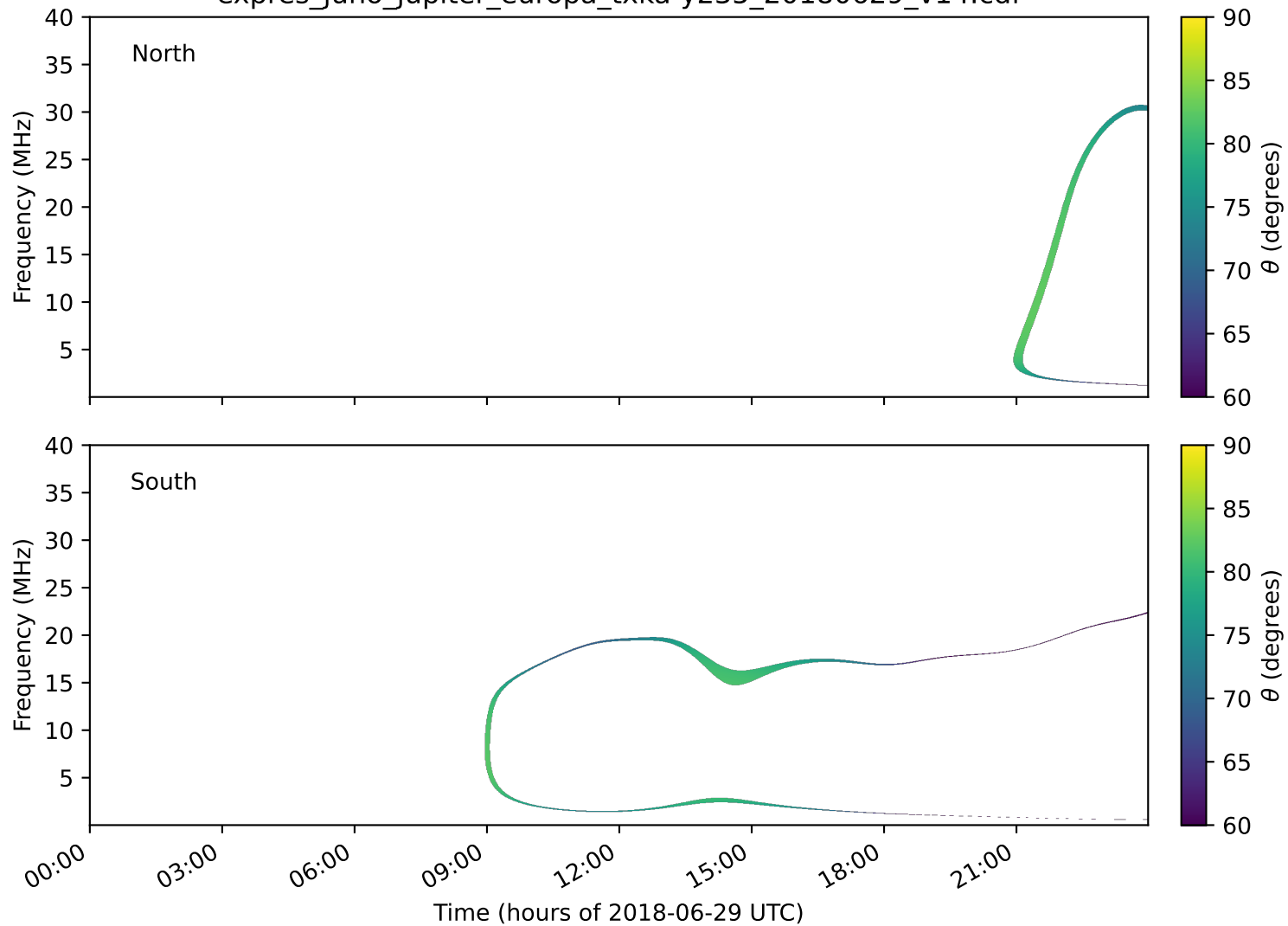
expres_juno_jupiter_europa_txka-y235_20180629_v14.cdf
