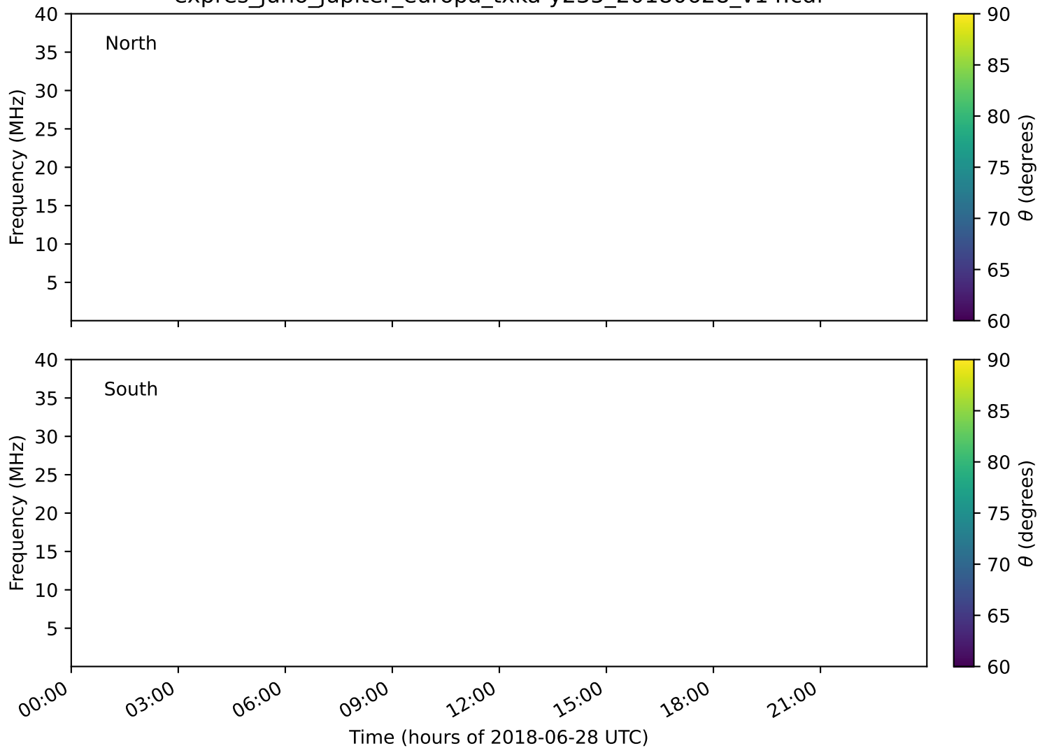
expres_juno_jupiter_europa_txka-y235_20180628_v14.cdf
