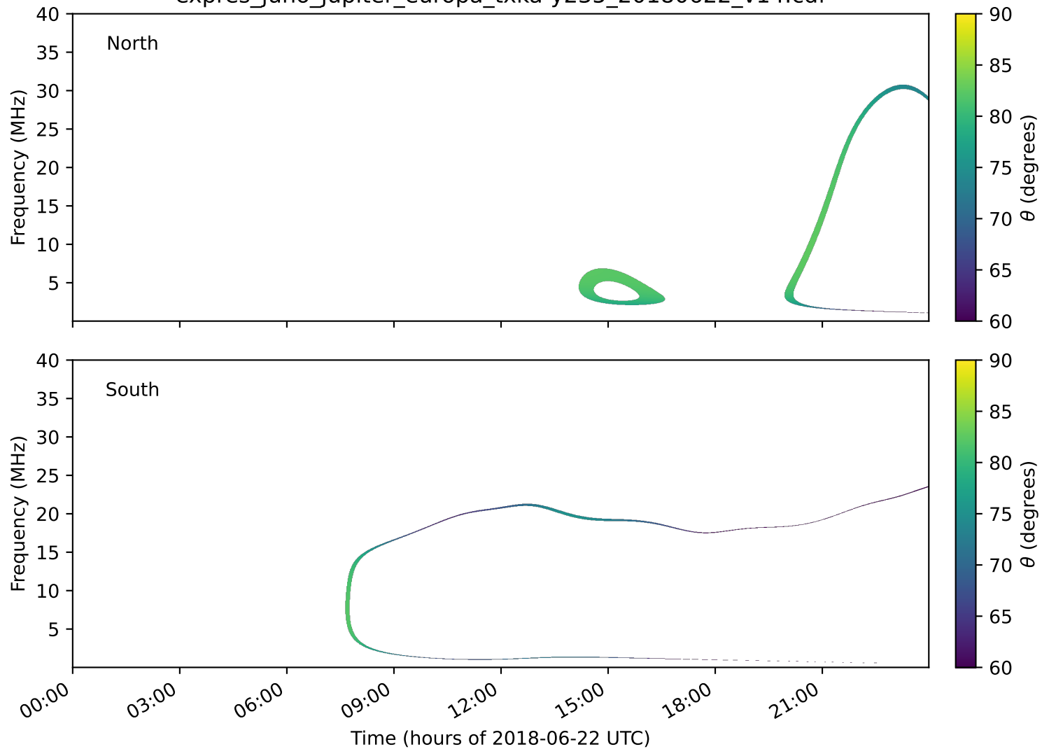
expres_juno_jupiter_europa_txka-y235_20180622_v14.cdf
