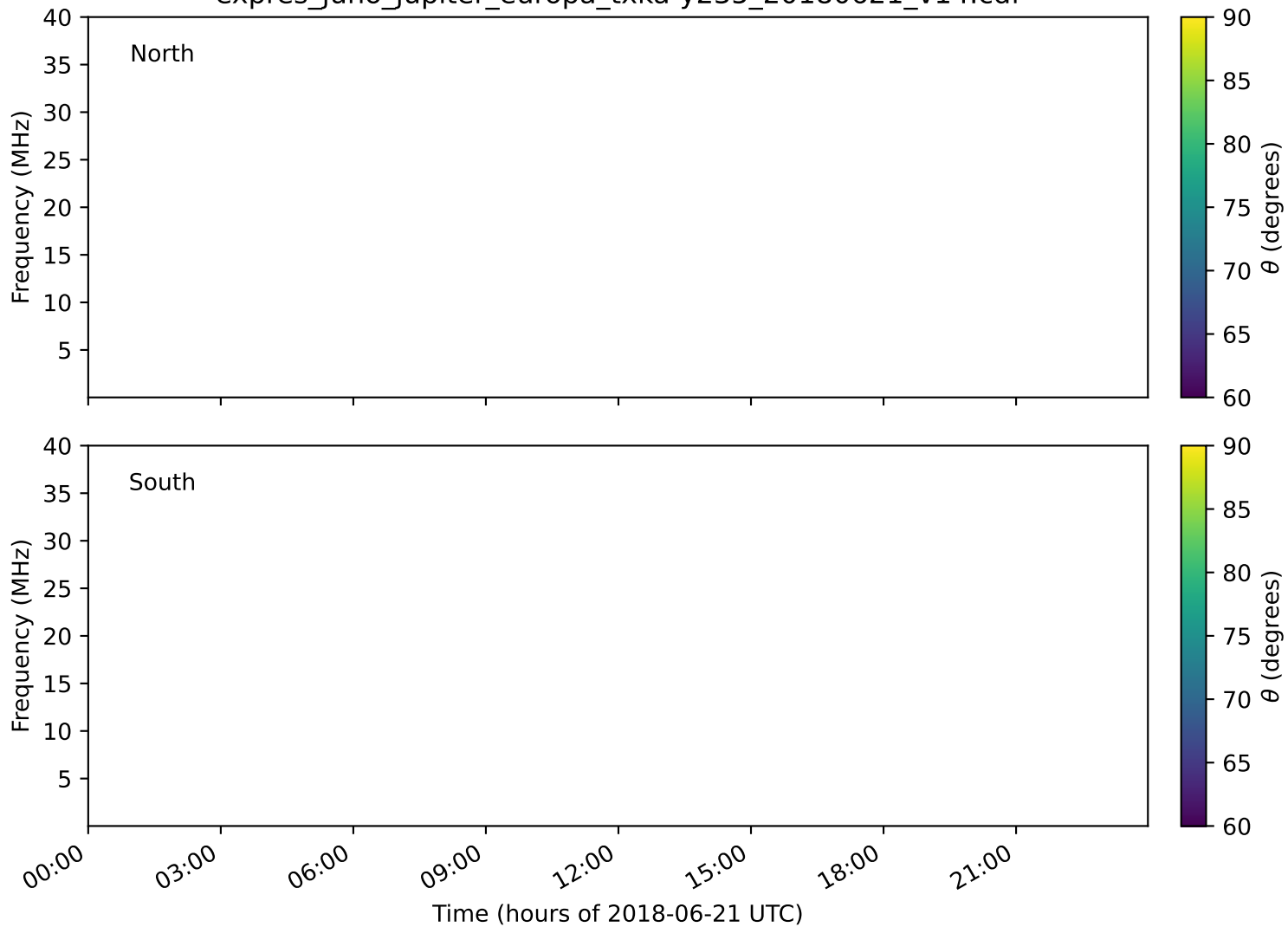
expres_juno_jupiter_europa_txka-y235_20180621_v14.cdf
