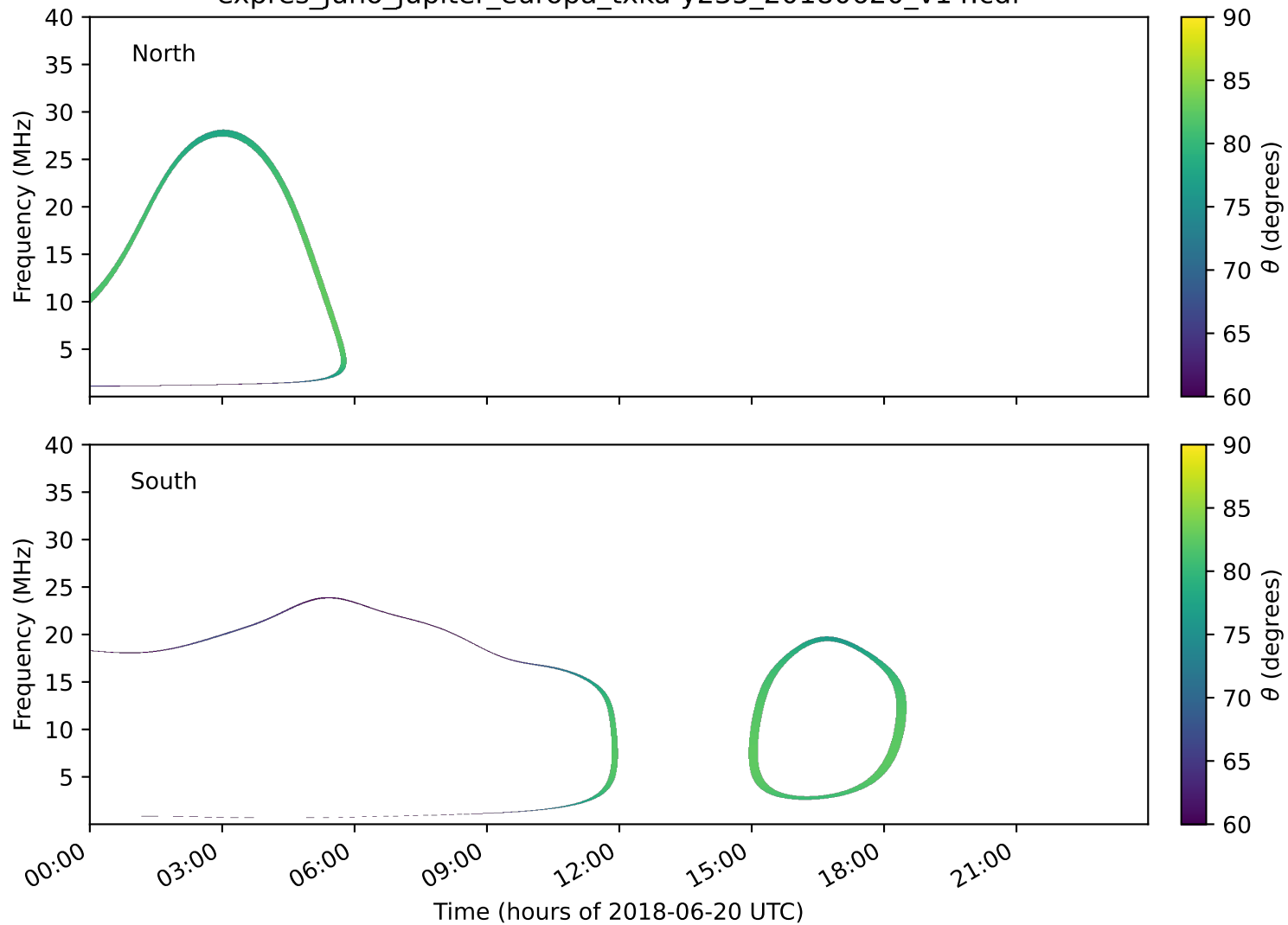
expres_juno_jupiter_europa_txka-y235_20180620_v14.cdf
