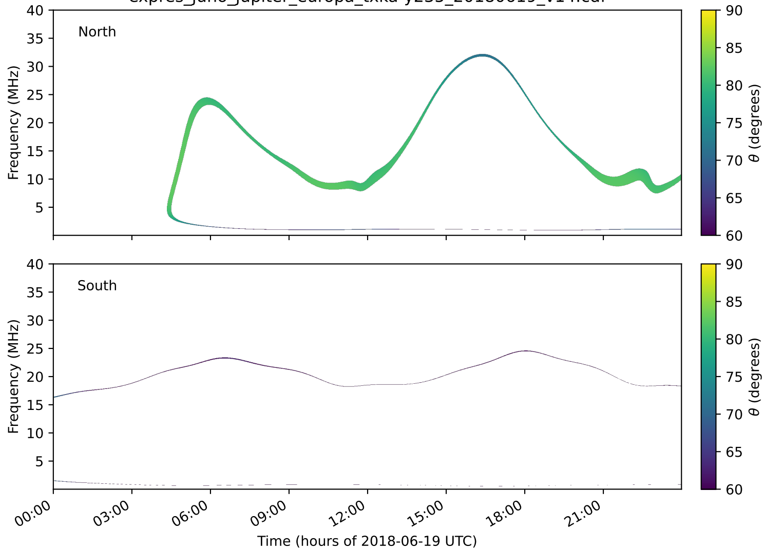
expres_juno_jupiter_europa_txka-y235_20180619_v14.cdf
