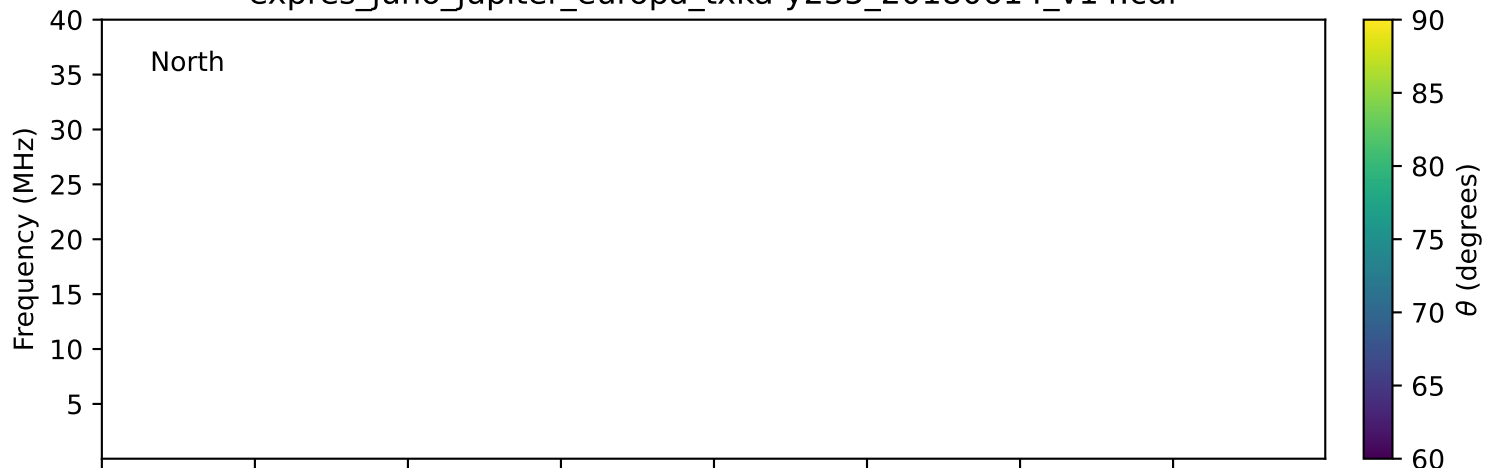
expres_juno_jupiter_europa_txka-y235_20180614_v14.cdf
