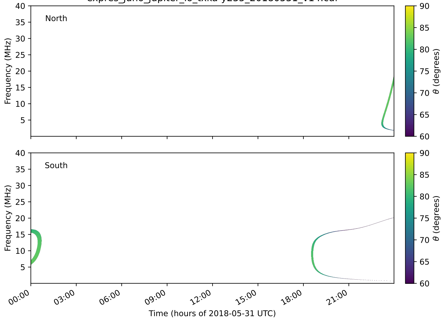
expres_juno_jupiter_io_txka-y235_20180531_v14.cdf
