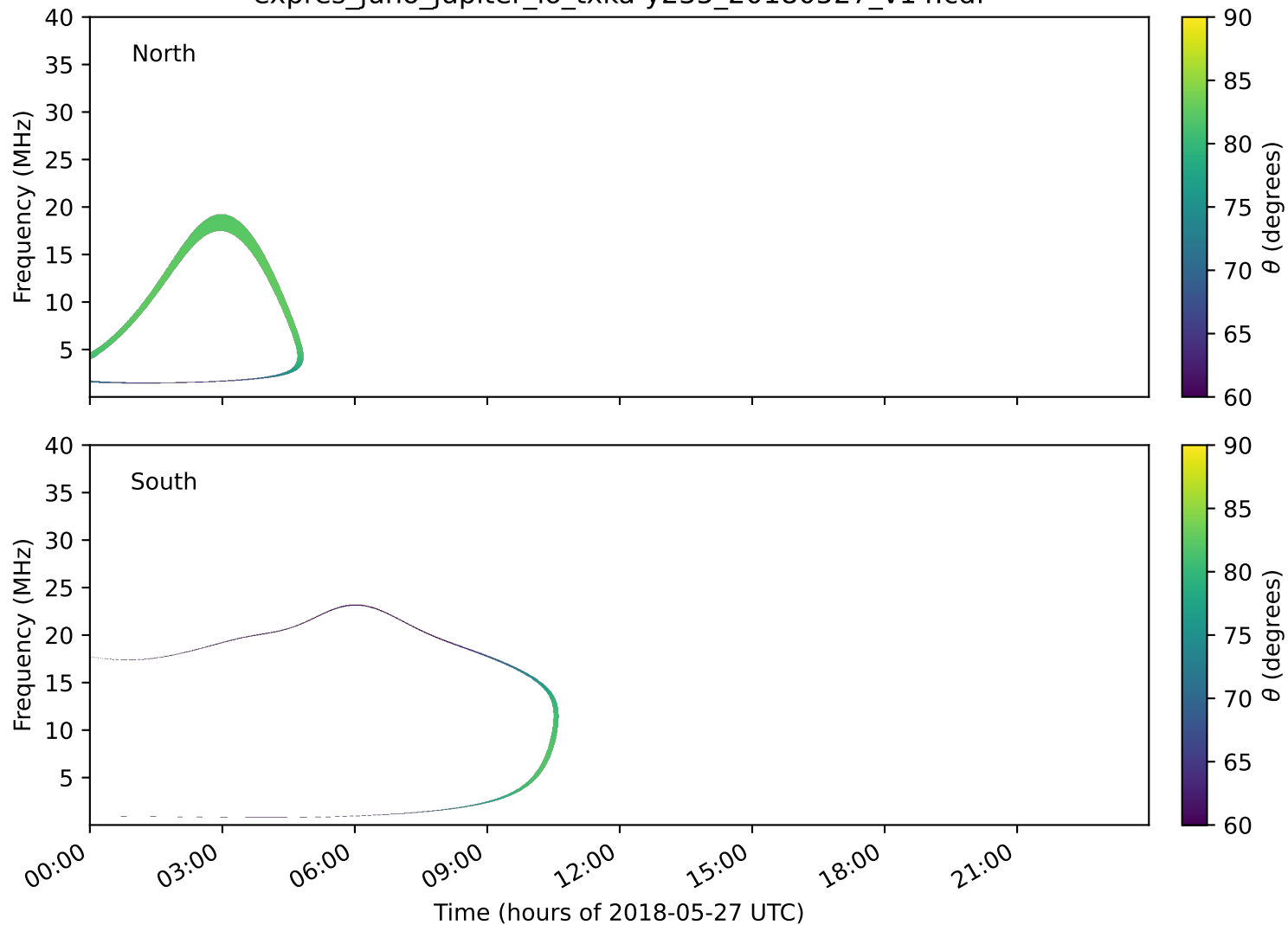
expres_juno_jupiter_io_txka-y235_20180527_v14.cdf
