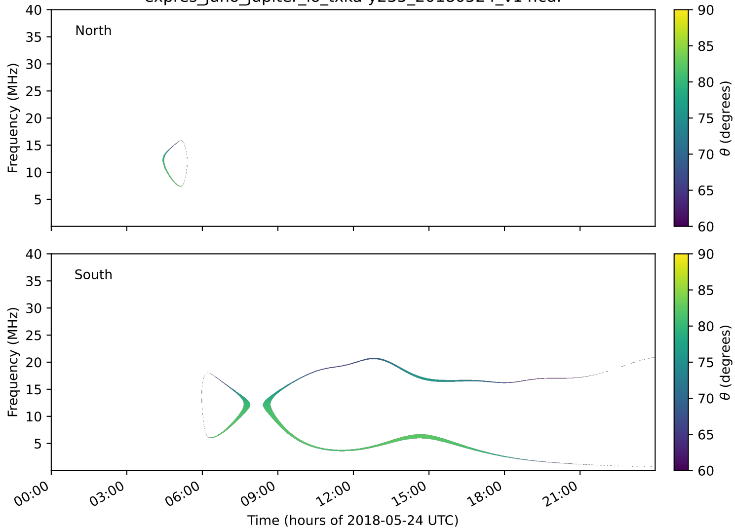
expres_juno_jupiter_io_txka-y235_20180524_v14.cdf
