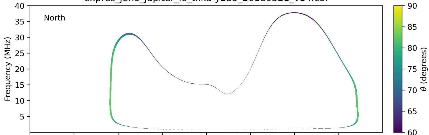
expres_juno_jupiter_io_txka-y235_20180521_v14.cdf
