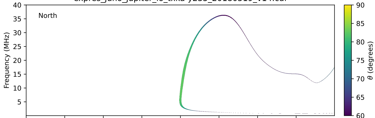
expres_juno_jupiter_io_txka-y235_20180519_v14.cdf
