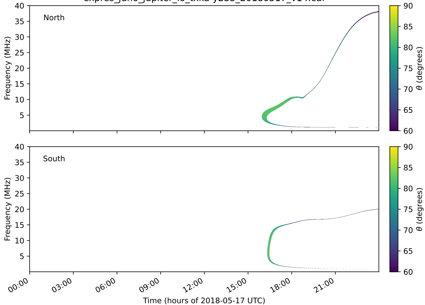
expres_juno_jupiter_io_txka-y235_20180517_v14.cdf
